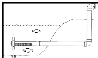
How a Dry hydrant works
