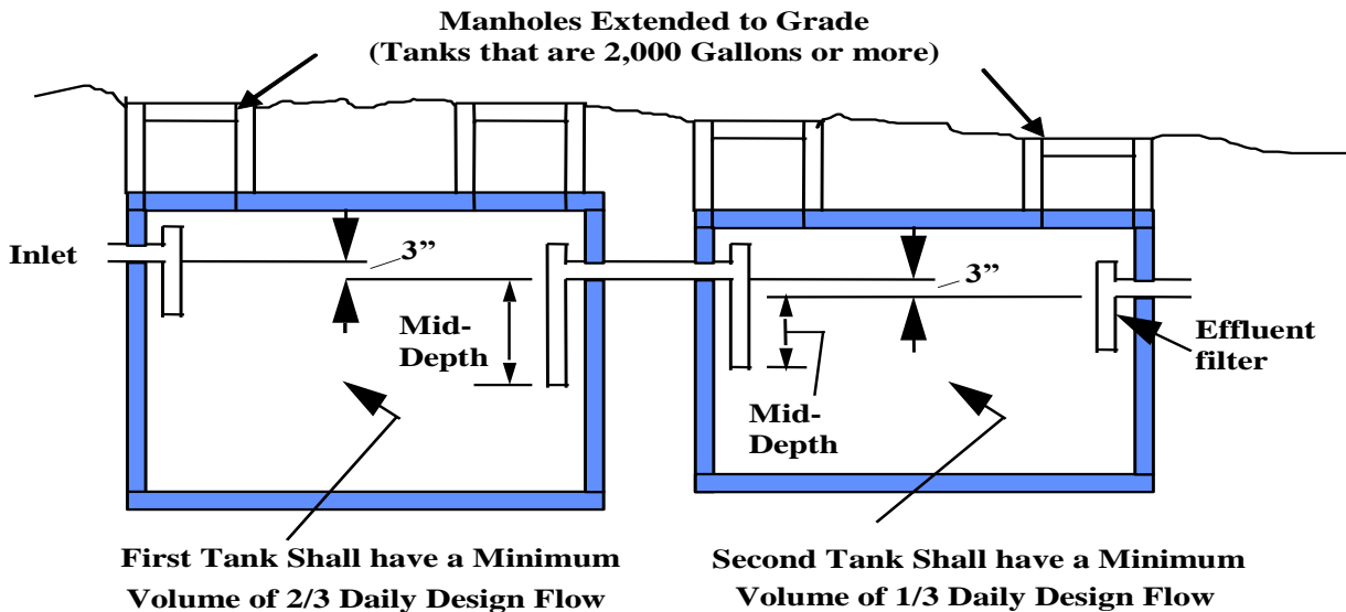
Figure 5 – Septic Tanks in Series
