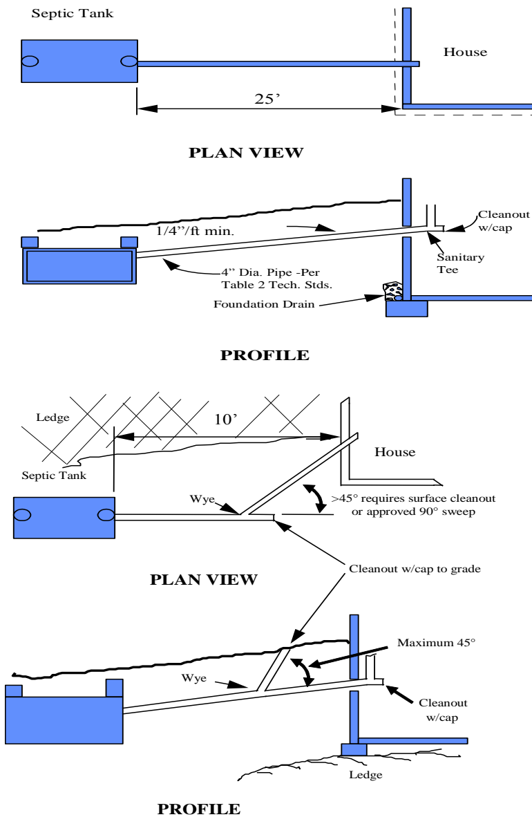
Figure 1 - Building Sewers
