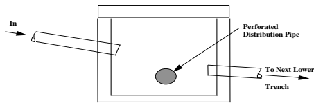
High - Level Overflow Dist. Box
