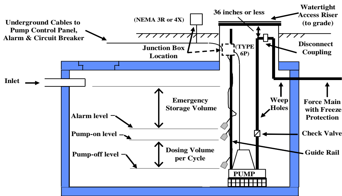
Figure 11 - Pump Chamber
