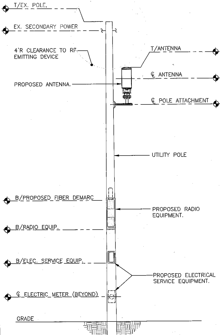
TYP. SIDE ARM MOUNT POLE ELEVATION
