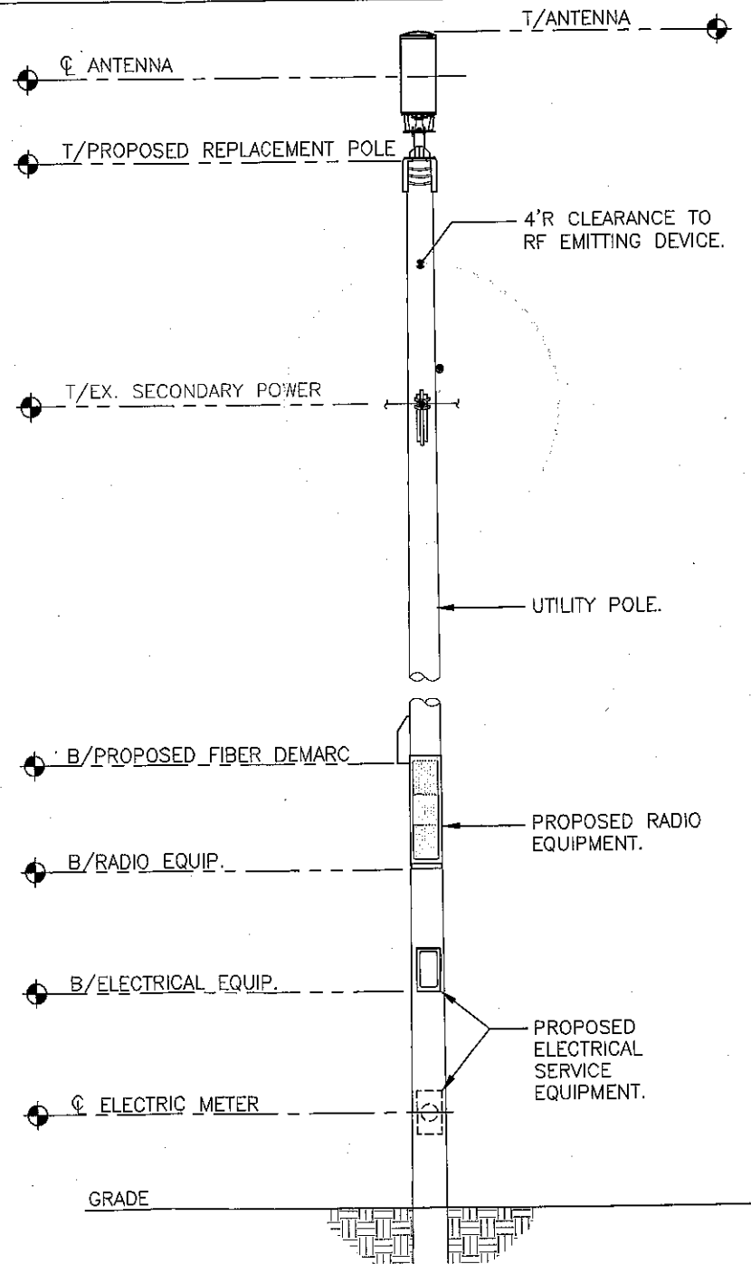
TYP. TOP MOUNT POLE ELEVATION
